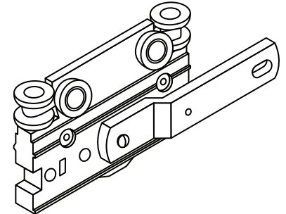
Baton Master Carrier - L.H. 8400-09
