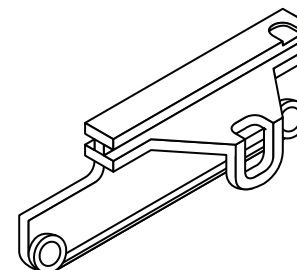
Snap Pleat Master Carrier - R.H. 8300-08
