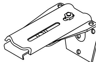
Wall Bracket 3" 8300-22
