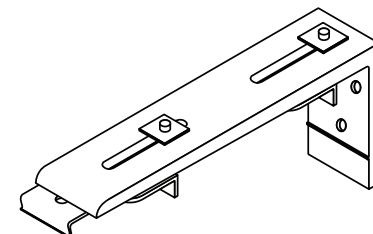
6" Wall Bracket 8100-45
