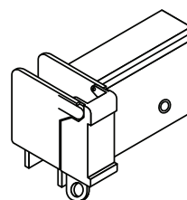
Ball Bearing Pulley - L.H. 8100-32
