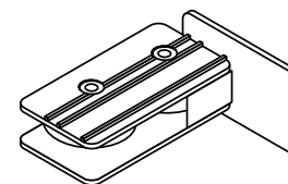
One-Way Draw Pulley - L.H. 8100-35
