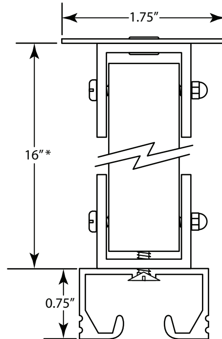
Twist Lock Carrier 7000-19
